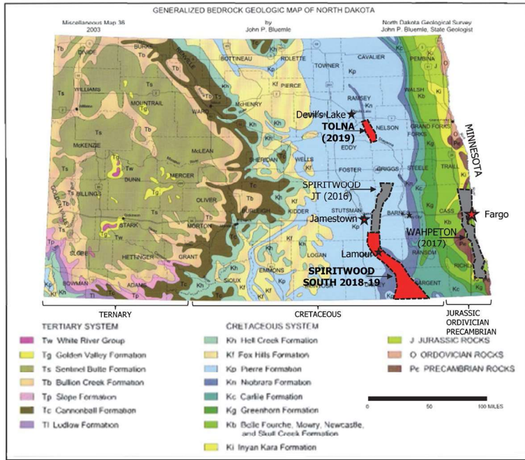
Figure 2 - Bedrock geology of North Dakota and approximate locations of Spiritwood-Tolna VTEM surveys and previous surveys for NDSWC (geology map after Bluemle, 2003).
