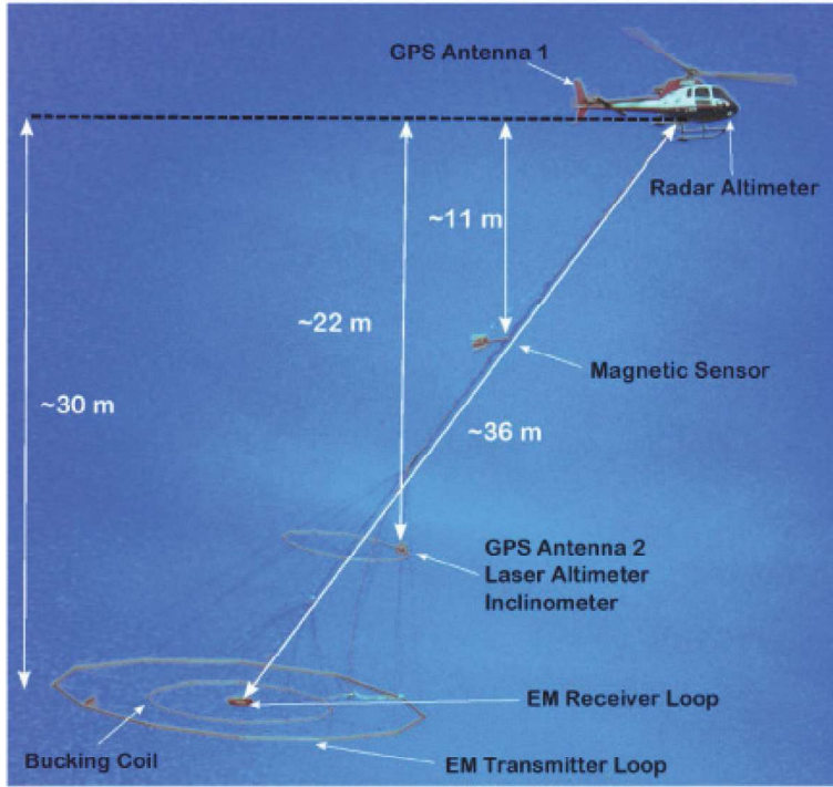
Figure 4 – VTEM ET (Early Time) time-domain electromagnetic system configuration.
