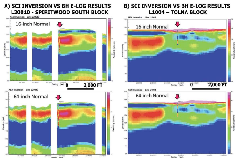
Figure 7: A comparison of the SCI inversions of test lines versus borehole E-logs for both the 16-inch and 64-inch normal for A) line L20010 flown over test hole 130775 within the Spiritwood South block, and B) line L1004 flown over test hole 130792 within the Tolna block. Test holes shown with red arrows. Resistivity range is 10-50 ohm-m.
