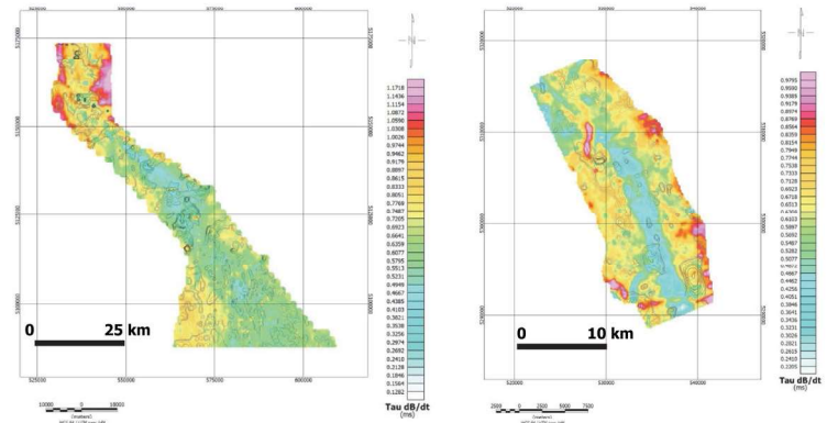
Figure 6: VTEM dBZ/dt EM time-constant (Tau) and calculated magnetic vertical gradient (CVG) contours for: A) Spiritwood South block (left) and B) Tolna block (right).
