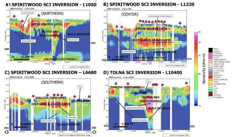
Figure 8: A comparison of the SCI inversions for east-west lines versus lithology for: A) line L1050 (north), B) L1220 (center) and L6680 (south) within the Spiritwood South block, and D) line L10400 within the Tolna block. Showing boreholes (red arrows) with lithology within 1/4 of a mile of the flight path. DOI traces shown at bottom of sections.
