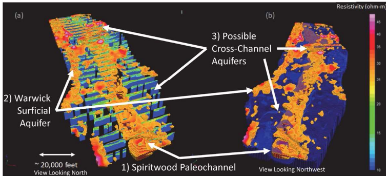
Figure 9: 3D voxel views of SCI Inversion results: A) Spiritwood South block, showing three 'chair'-clipped zooms of areas of interest within the survey highlighting the 25 to 50 ohm-m deposits. B) Tolna block, showing features of interest and highlighting >23 ohm-m resistivities. Vertical Exaggeration is 15x. Resistivity range 10-50 ohm-m.
