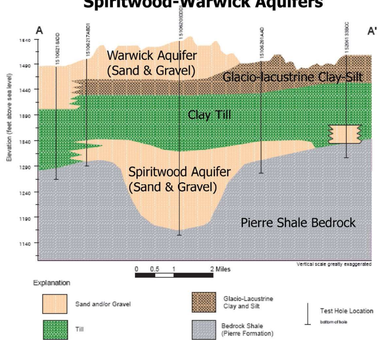
Figure 3 - Geologic cross-section across Spiritwood-Warwick aquifers (after Patch and Honeyman, 2005).
