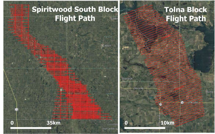
Figure 5: VTEM ET flight path (as flown) over Spiritwood South block (left) and Tolna block (right).
