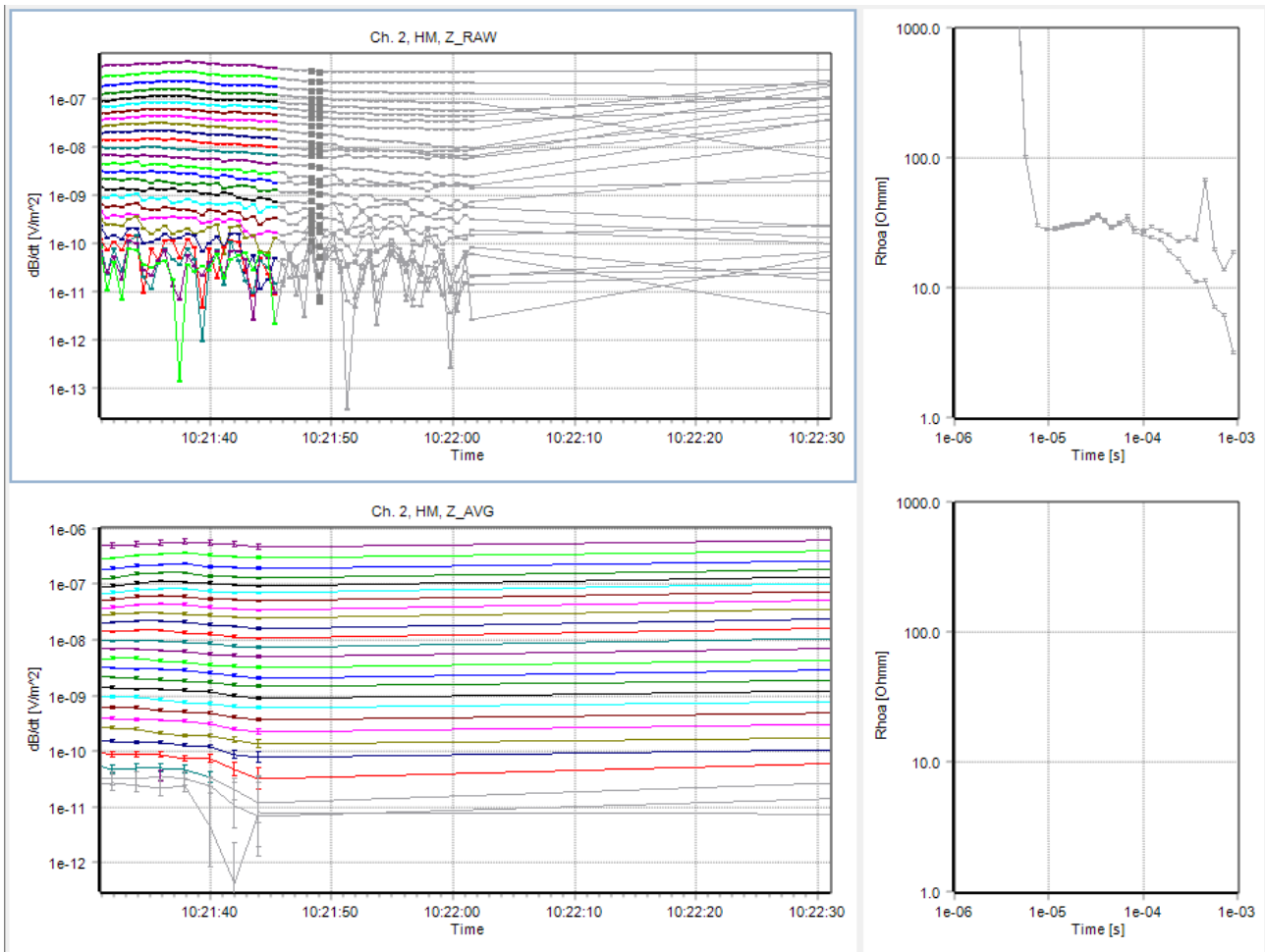
Figure 5.1a: Example of some coupled data, and how they have been removed. The sounding plot clearly shows that the coupling still is present at the selected positions, even though the lines on the data plot at first glance might look fine. Looking closer one can see how the lines diverging or converging to form the bumps that we see on the sounding plot. With TEMPEST the equivalent sounding plot would show B field.
