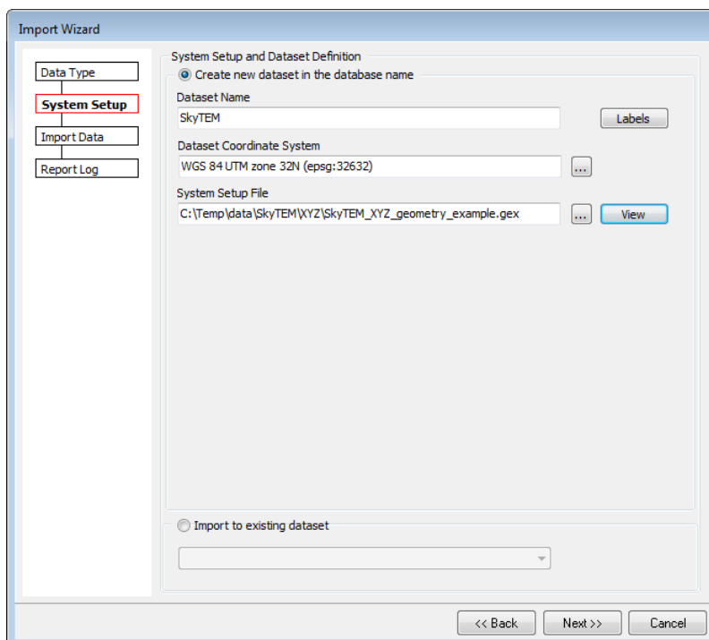
Figure 1.3a: SkyTEM xyz data import – System Setup Page
